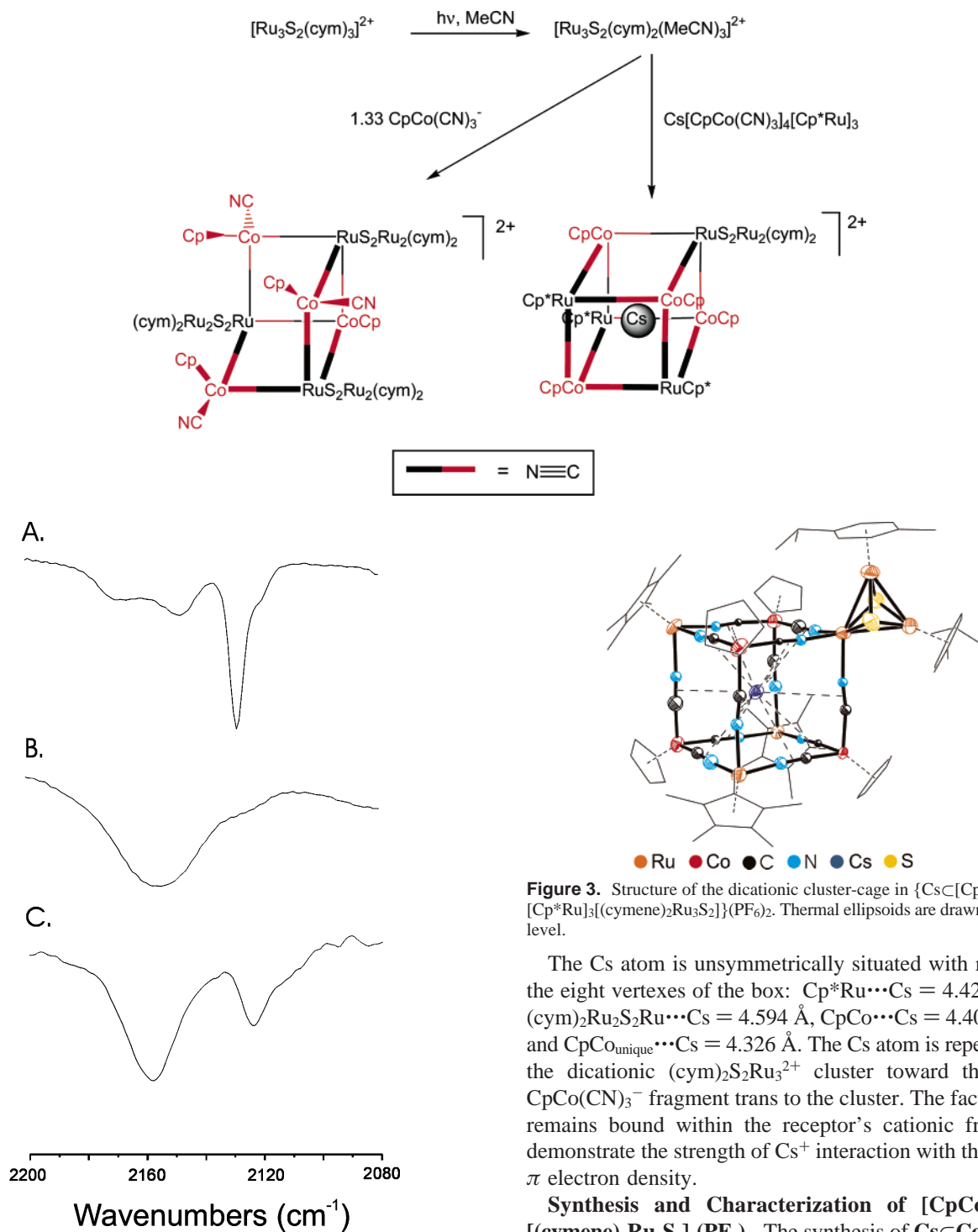
Figure 2. IR spectra (MeCN) in the \nu_{\text{CN}} region for \text{CsCCo}_4\text{Ru}_3 (A), \text{CsCCo}_4\text{Ru}_6\text{S}_2^{2+} (B), and \text{Co}_4\text{Ru}_9\text{S}_6^{2+} (C).
