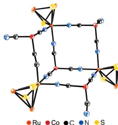
Figure 5. Structure of the dicationic cluster-cage in \{[\text{CpCo}(\text{CN})_3]_4-[(\text{cymene})_2\text{Ru}_3\text{S}_2]_3\}(\text{PF}_6)_2 ; the hydrocarbon ligands are omitted for clarity. Thermal ellipsoids are drawn at the 25% level.
